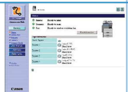
Remote UI
